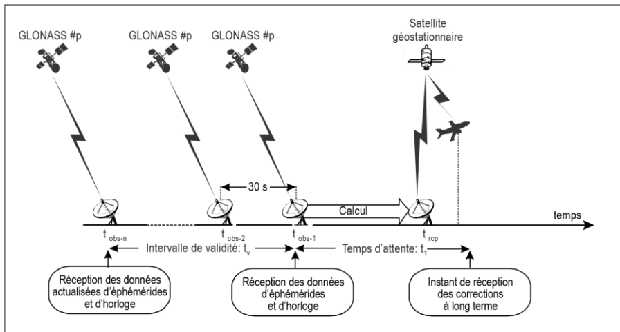
Figure D-3. Temps GLONASS
