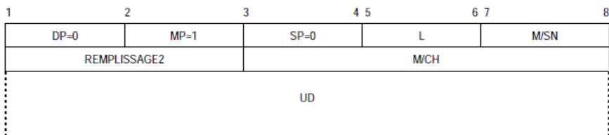
Figure 5-22. Paquet MSP LONG
