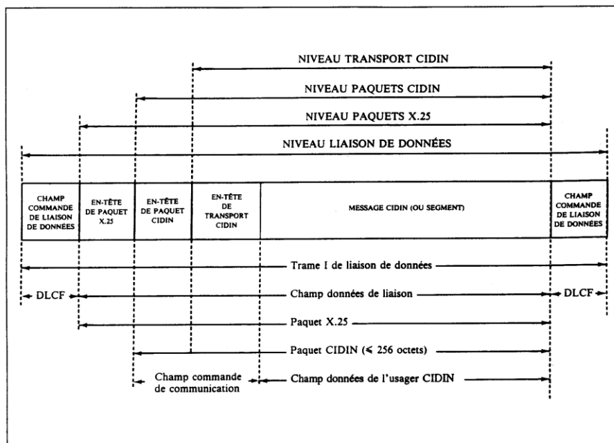
Figure 8-2. Terminologie CIDIN
