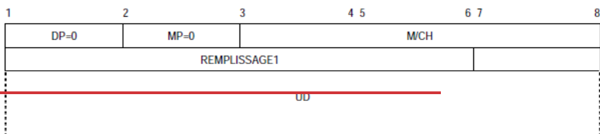
Figure 5-21. Paquet MSP COURT
