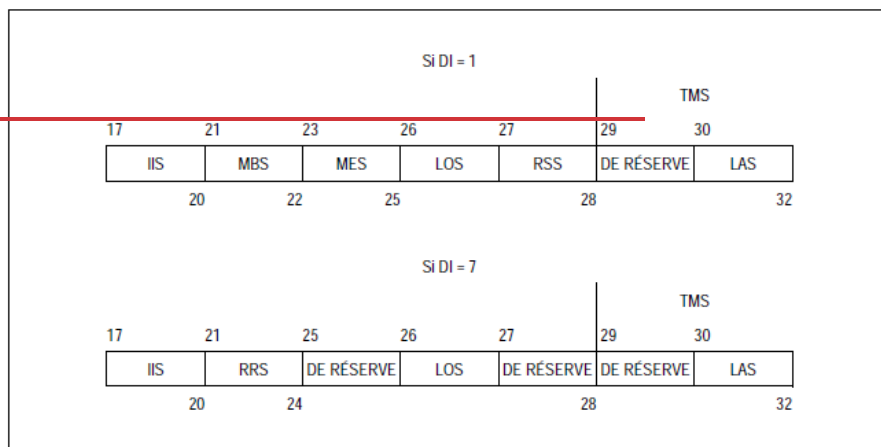
Figure 5-1. Structure du champ SD
