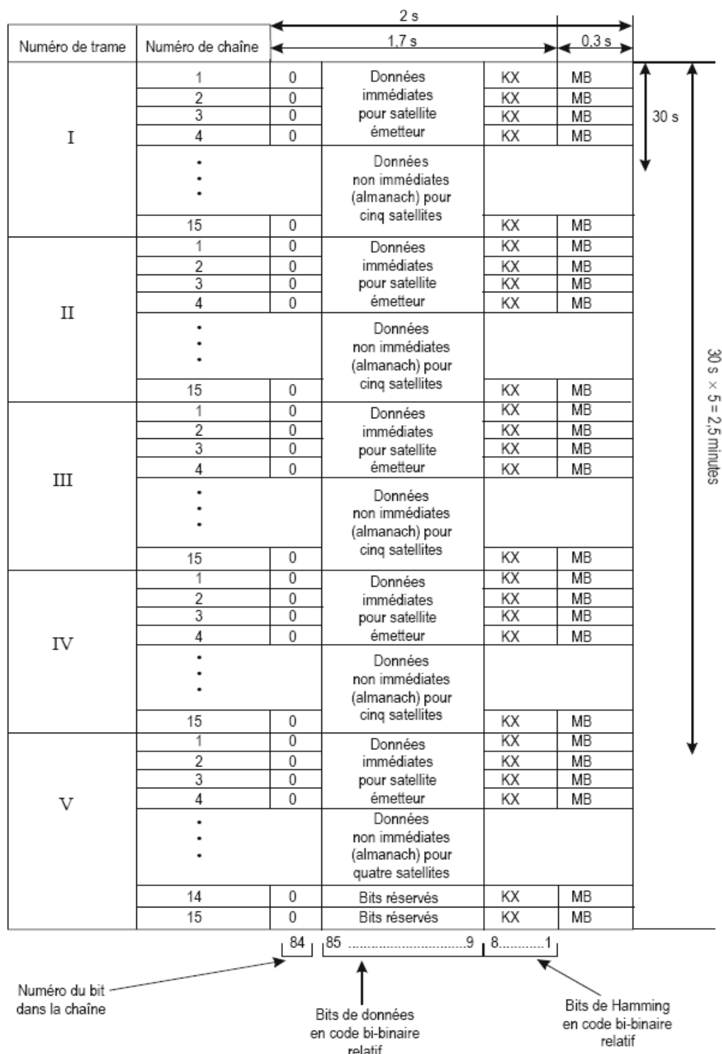
Figure B-7. Structure de la superframe
